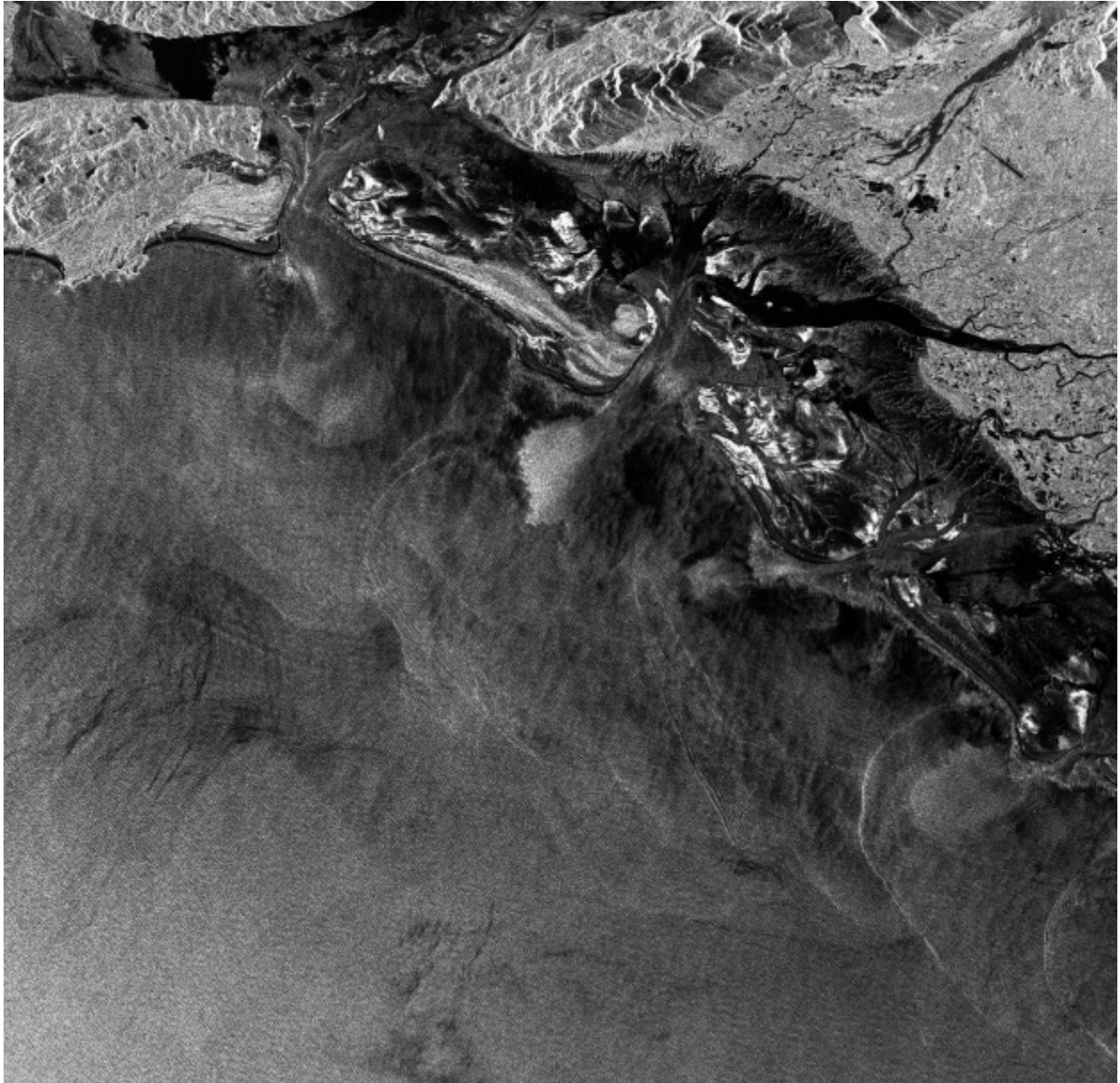
Figure 2. Radarsat standard mode image showing internal wave signatures in Prince William Sound, Alaska. Image was acquired on June 11, 1998, 03:06 GMT. Image is 45 km x 45 km centered at 60.0 0 N., 146.0 0 W. [Image from the Alaska SAR DEMO Imagery Manual - October 1999 courtesy of NOAA NESDIS ©CSA 1998]
