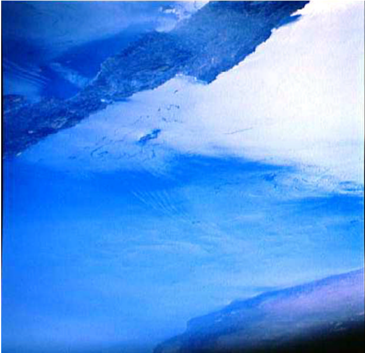
Figure 1. Space Shuttle Photograph (STS41G-36-23) collected on October 6, 1984 at GMT 11:57 centered near 35.0^{\circ} N, 25.0^{\circ} E. Image shows internal waves on either side of the Isle of Crete propagating westward. Image Courtesy of Earth Sciences and Image Analysis Laboratory, NASA Johnson Space Center ( http://eol.jsc.nasa.gov ).
